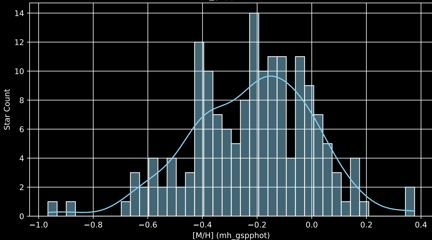
APOGEE DR17 Field: [053+35_MGA [M/H] (mh_gspphot) (n= 164)
