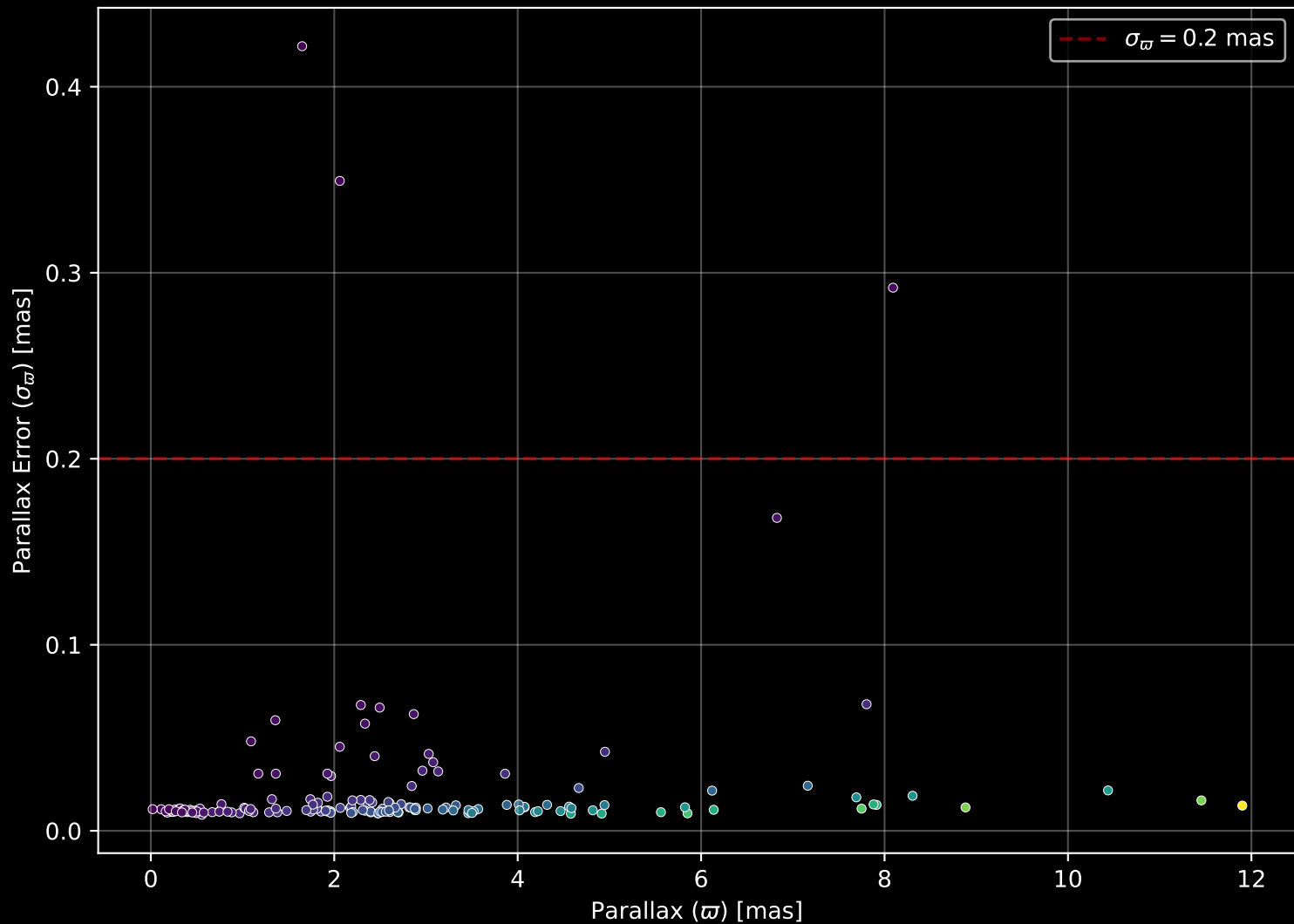
APOGEE DR17 Field: [053+35_MGA] Parallax Quality (n= 166)
