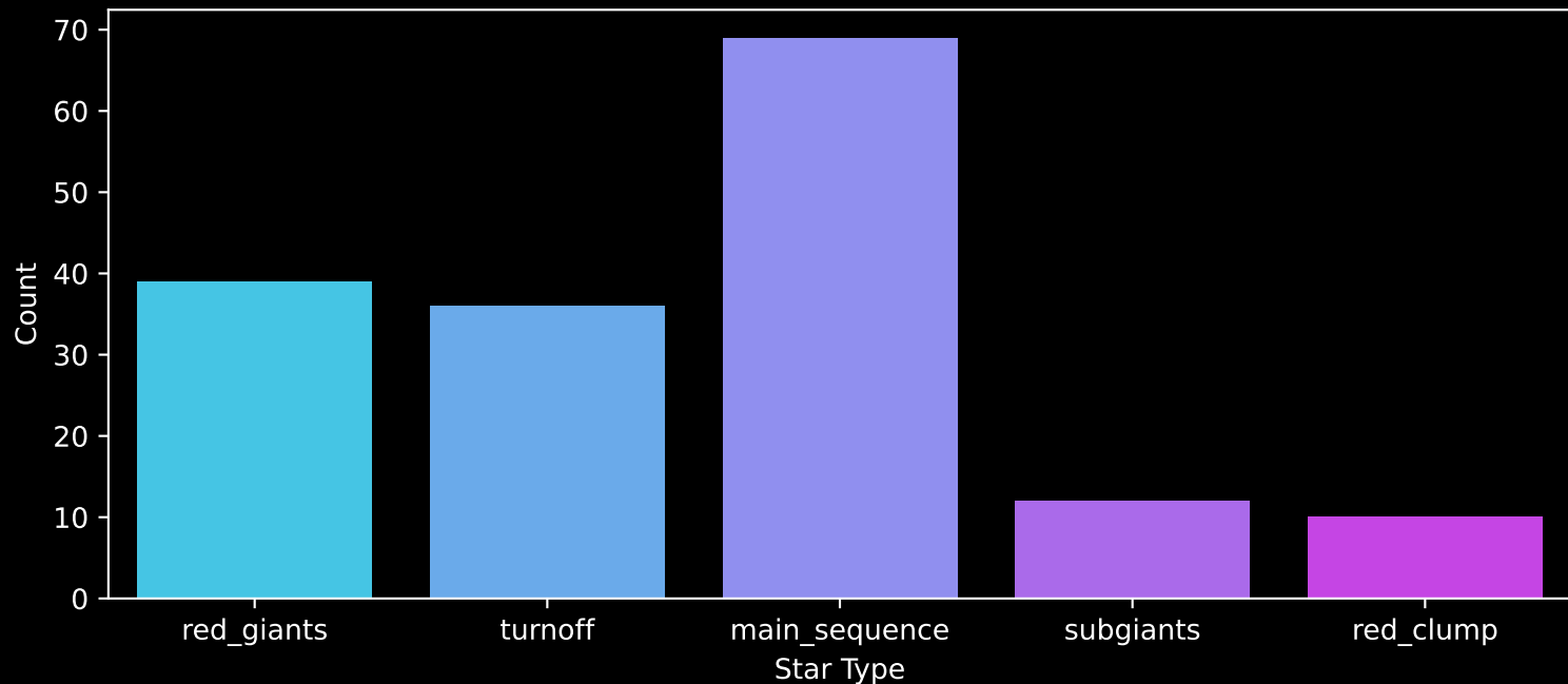
APOGEE DR17 Field: [053+35_MGA] Count plot of Star Type
