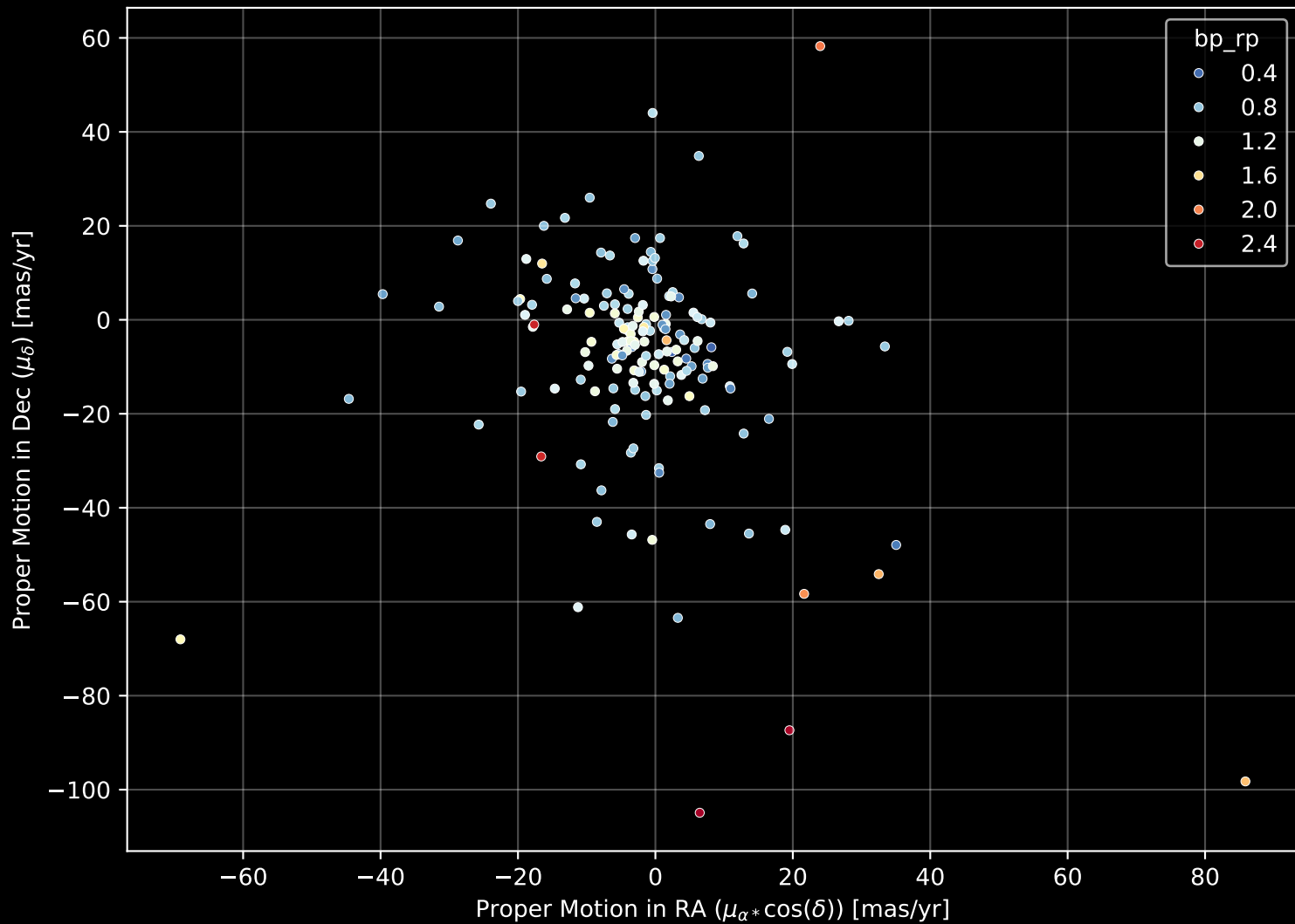
APOGEE DR17 Field: [053+35_MGA] Proper Motion Diagram (n= 166)
