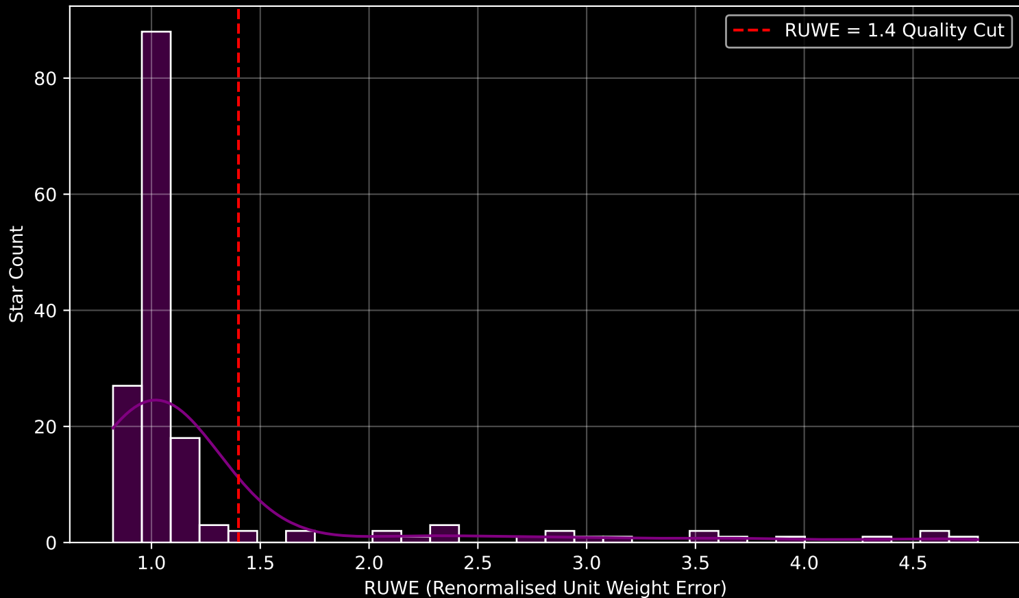
GAPOGEE DR17 Field [053+35_MGA] RUWE Distribution (n= 159)
